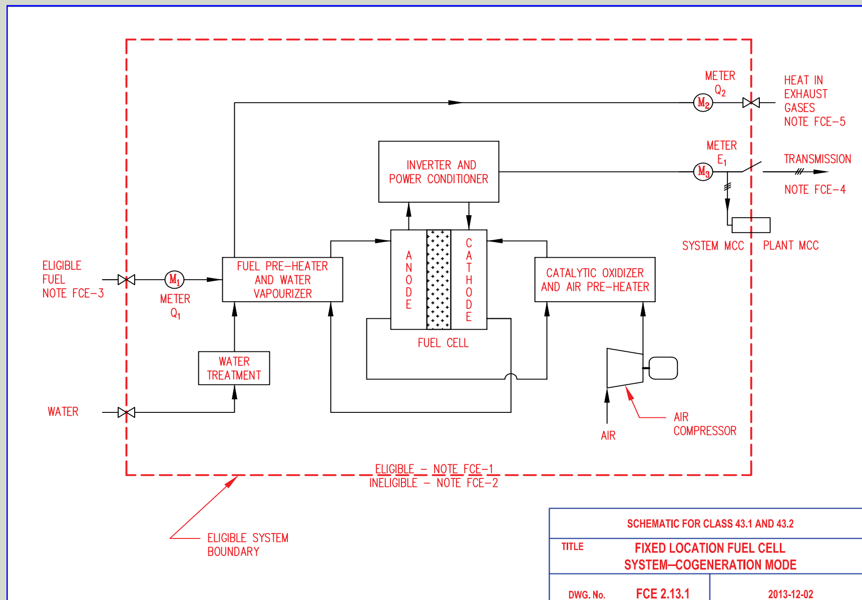
FCE 2.13.1 Fixed Location Fuel Cell System—Cogeneration Mode
