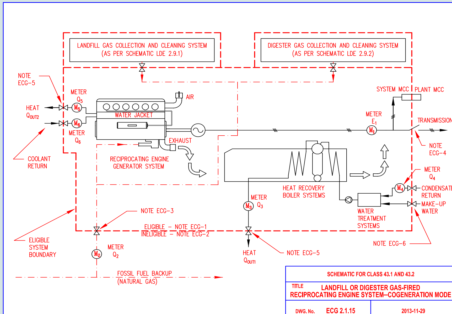
ECG 2.1.15 Landfill or Digester Gas-Fired Reciprocating Engine System—Cogeneration Mode
