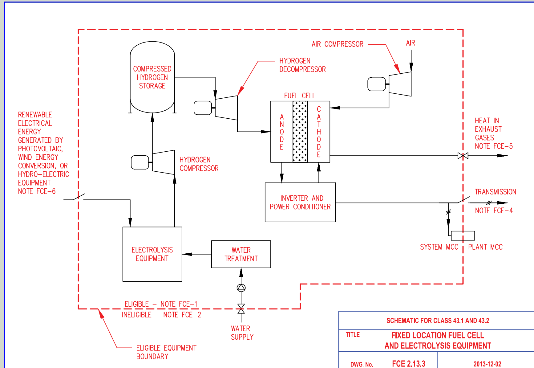
FCE 2.13.3 Fixed Location Fuel Cell and Electrolysis Equipment
