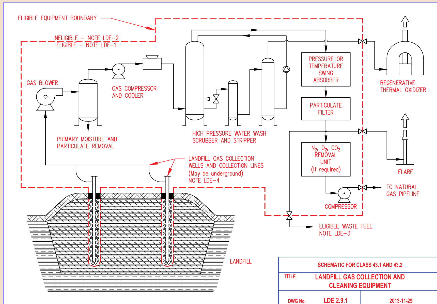
LDE 2.9.1 Landfill Gas Collection and Cleaning Equipment
